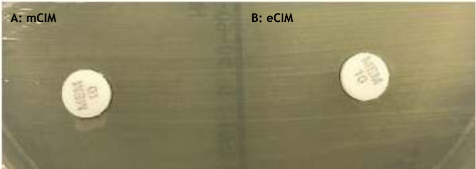
Figure 3D. mCIM and eCIM Test Interpretation: Positive mCIM and Negative eCIM. “A” shows an mCIM positive result (zone diameter = 6 mm) and “B” shows an eCIM negative result (zone diameter = 6 mm). Serine carbapenemases are not inhibited by EDTA and demonstrate a \leq 4 -mm increase in zone diameter for eCIM vs zone diameter for mCIM.
